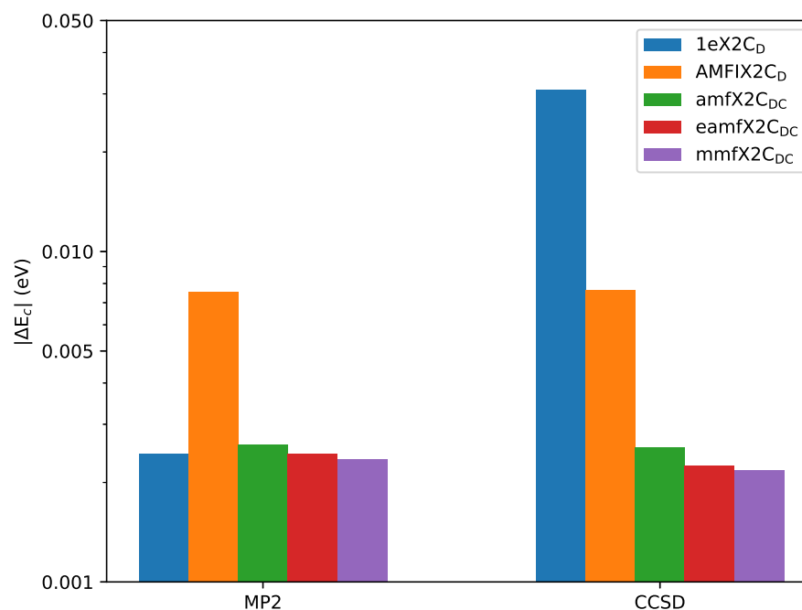
Figure 2: Absolute MP2 and CCSD correlation energies differences between 4 DC ( |\Delta E_c| , in eV), for different Hamiltonian calculated for \text{CnF}_6 with the same computational setup as for the EOM-CCSD core-ionization energies. Note that the scale on the y-axis is logarithmic. Further computational details are given in the text.
