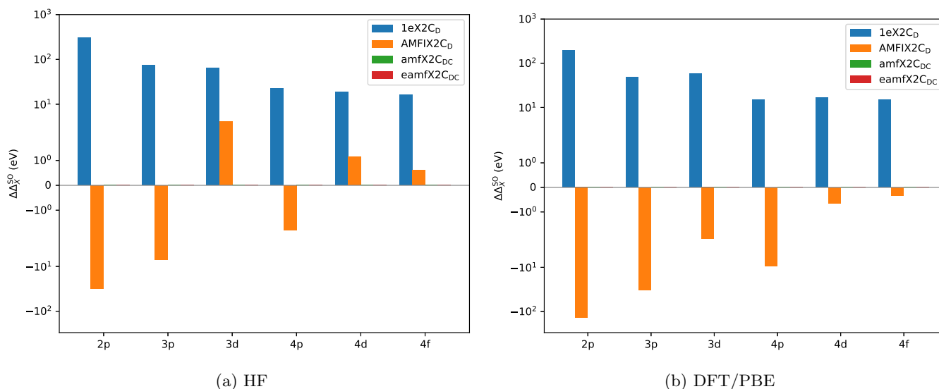
Figure 1: Differences of spin-orbit splittings ( \Delta_X^{\text{SO}} ) of the inner-core to outer-core Og-atomic-like shells in \text{Og}_2 with respect to the ^4\text{DC} reference values either within a HF approach (panel (a)) or a DFT/PBE approach (panel (b)). All data is compiled from the SCF spinor energies listed in Tables II and III, respectively. Energy differences are given in eV. Note that errors associated with the (e)amfX2C models are not visible in the figures.
