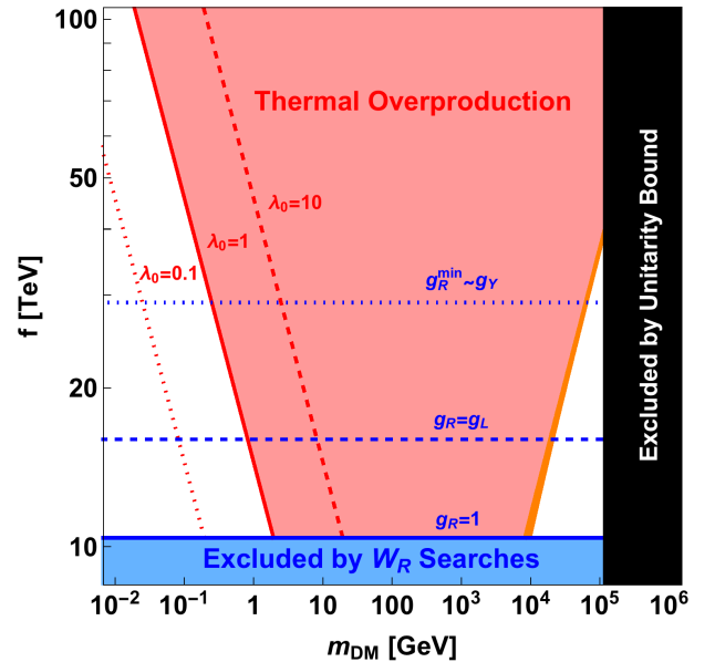
FIG. 1. Constraints on m_{DM} and the compositeness scale f \equiv f_L = f_R . The red shaded region is excluded by thermal overproduction, while an upper limit on m_{DM} \lesssim 110 \text{ TeV} comes from unitarity bounds [50]. The low mass limit of the excluded region depends on \lambda_0 , and we show three sample values. A lower limit on f comes from direct searches of W_R at colliders, which crucially depends on the value of g_R (we show three sample values: g_R = 1, g_L, g_Y , with the last being the minimum allowed value). The high m_{DM} edge of the red region has a mild dependence on g_R , illustrated by the thin orange band, moving to the right for larger g_R .
