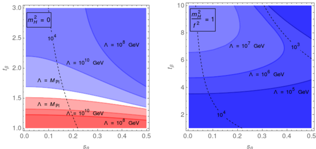
Figure 3. The blue (red) regions illustrate the vacuum instability (non-perturbativity) scale. The dashed lines show the values of \Lambda_{TC} = 4\pi f in GeV. Left panel: m_H^2 = 0 . On the boundaries of the regions, the vacuum is stable (couplings perturbative) up to \Lambda = M_{Pl} = 1.22 \cdot 10^{19} GeV, 10^{10} GeV, 10^8 GeV. Right panel: m_H^2/f^2 = 1 . On the boundaries of the regions, the vacuum is stable up to \Lambda = 10^7 GeV, 10^6 GeV, 10^5 GeV.
